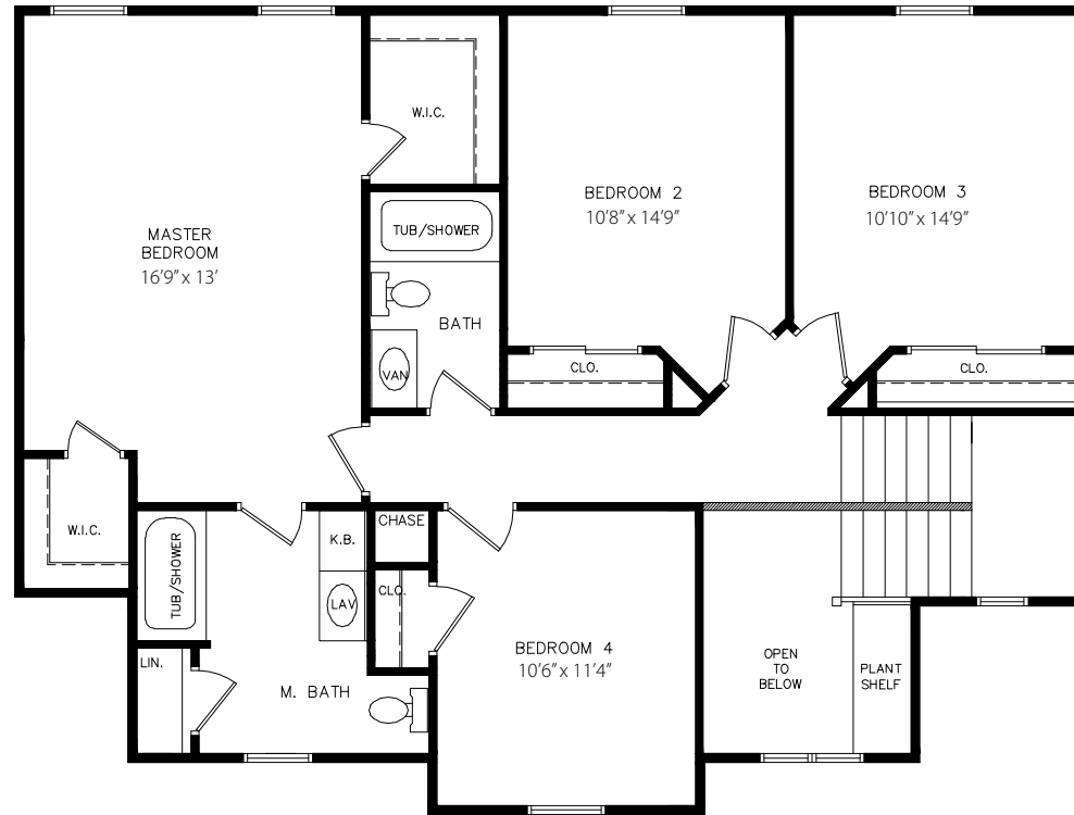
2nd FLOOR PLAN 1/8" = 1'-0"
