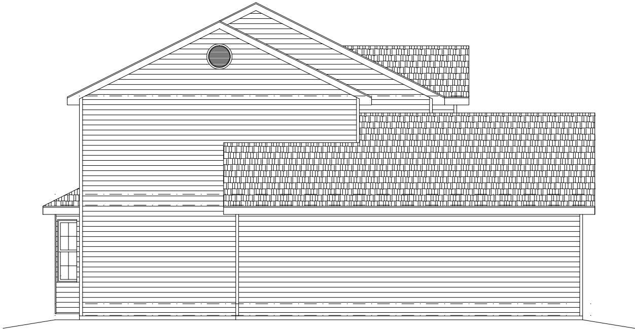
LEFT ELEVATION
