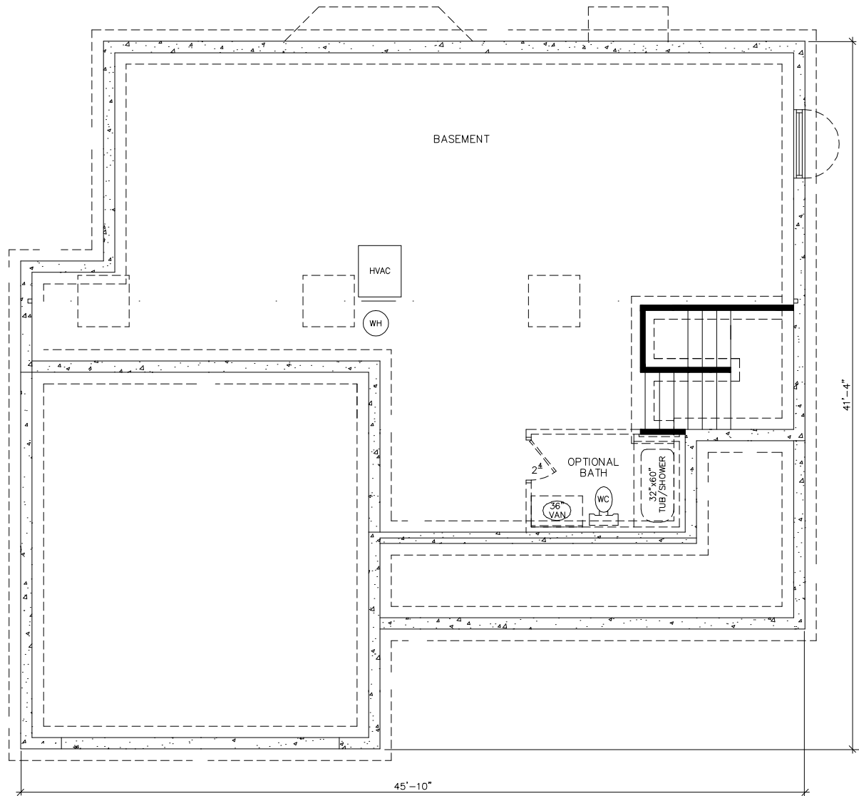
FOUNDATION PLAN
