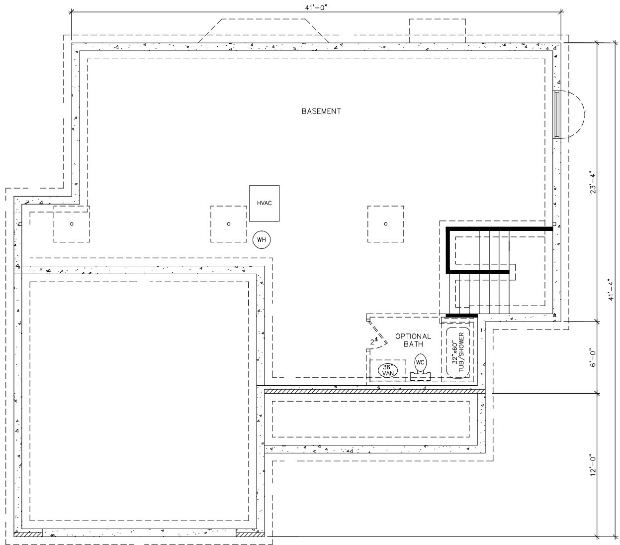
FOUNDATION PLAN
