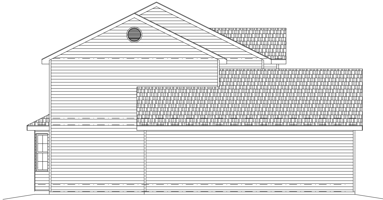
LEFT ELEVATION
