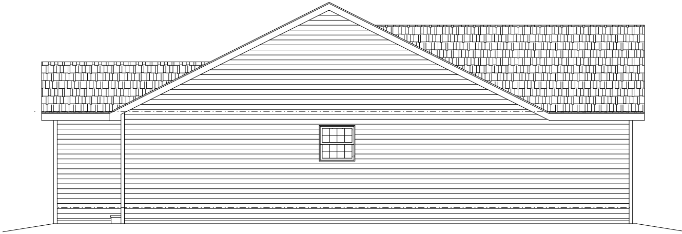
LEFT ELEVATION
