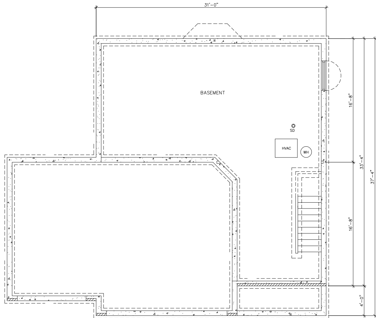
FOUNDATION PLAN
